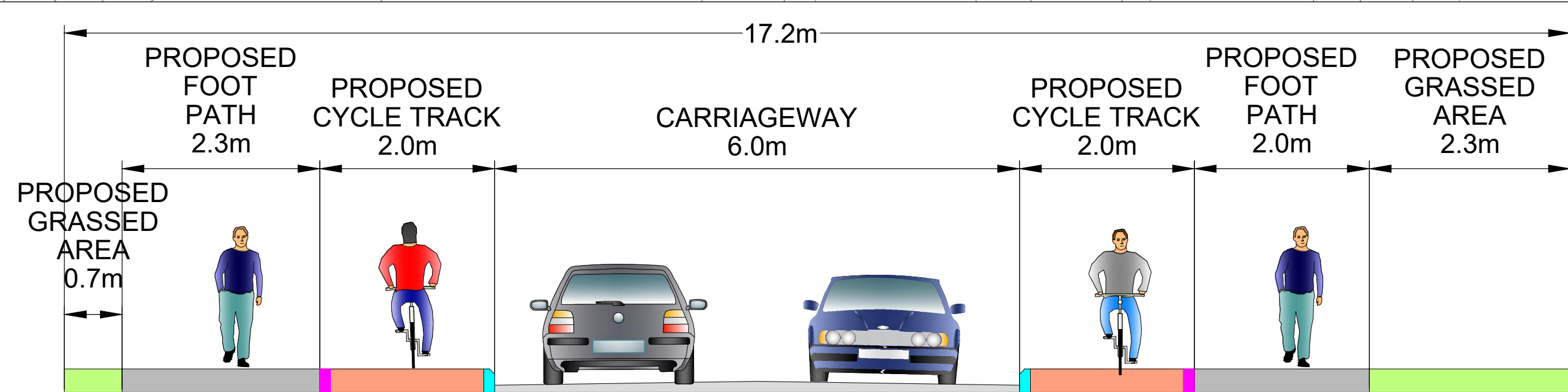
CROSS SECTION S-S
